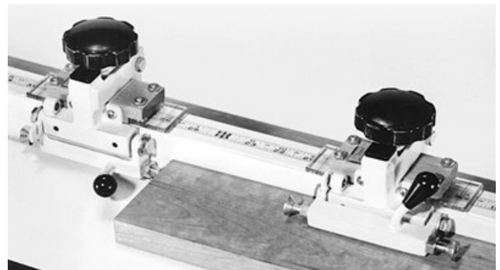
78-992 - Biesemeyer T-Square Dual Pointer Flip Stop
